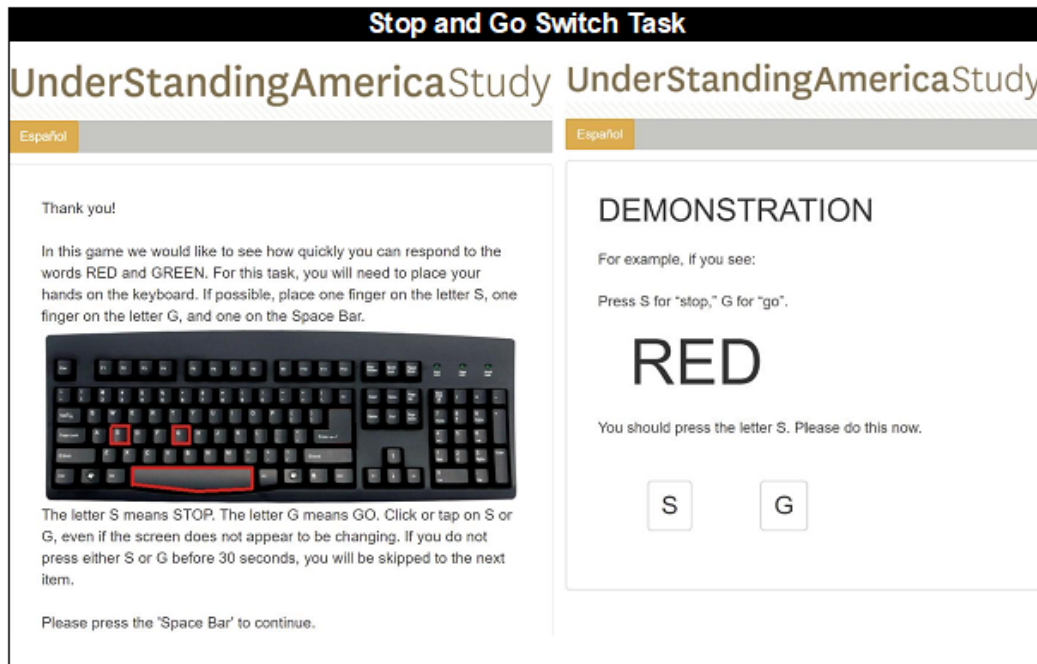
Figure 1: Example screens
